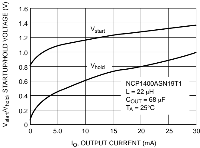
Figure 26. NCP1400ASN19T1 Operation Startup/Hold Voltage vs. Output Current
